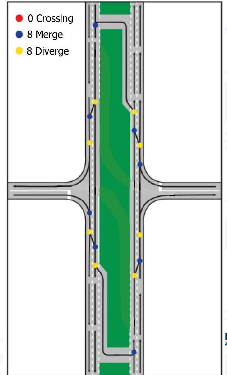
Median U-Turn Intersection
