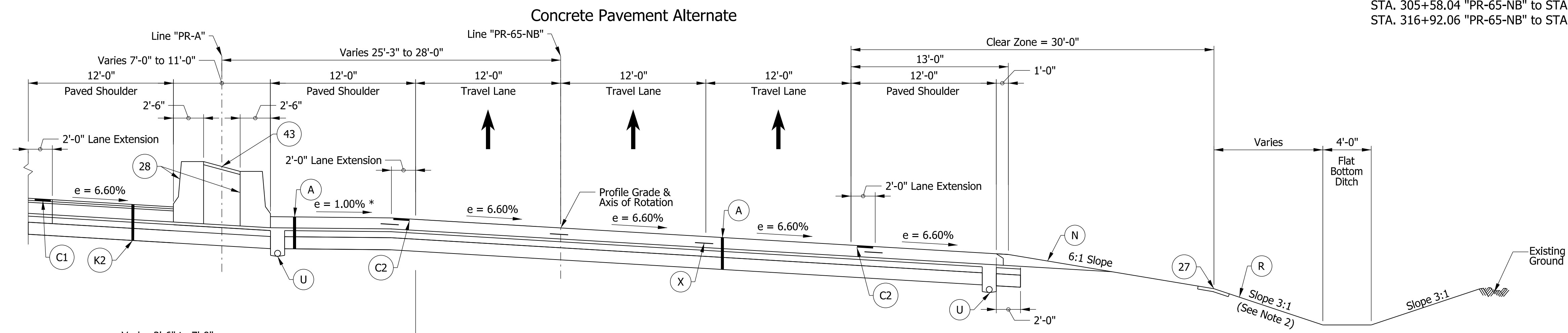
I-65 SUPERELEVATION TYPICAL SECTION NORTHBOUND A STA. 301+96.00 "PR-65-NB" to STA. 329+61.00 "PR-65-NB"
