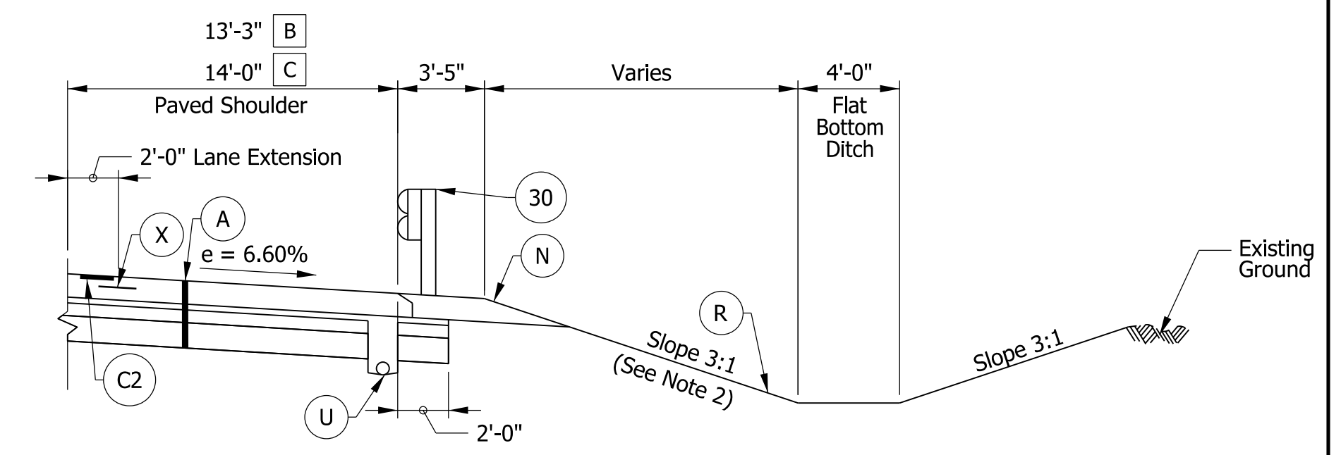
NB GUARDRAIL AND OUTSIDE SHOULDER DETAIL STA. 305+58.04 "PR-65-NB" to STA. 308+13.45 "PR-65-NB" B STA. 316+92.06 "PR-65-NB" to STA. 322+36.79 "PR-65-NB" C
