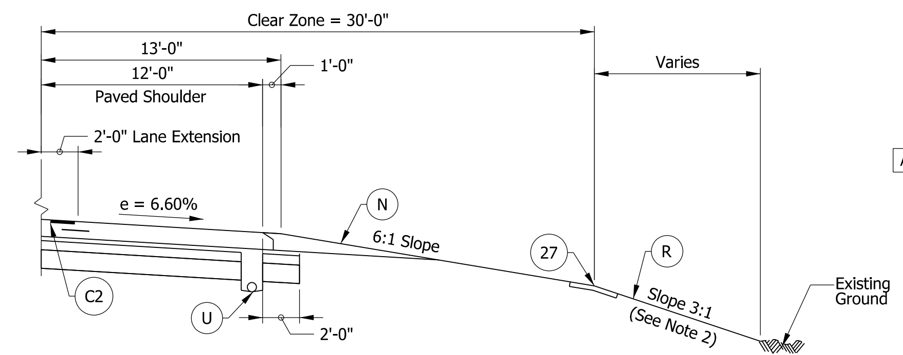
NB OUTSIDE SHOULDER DETAIL STA. 308+13.45 "PR-65-NB" to STA. 314+00.00 "PR-65-NB"
