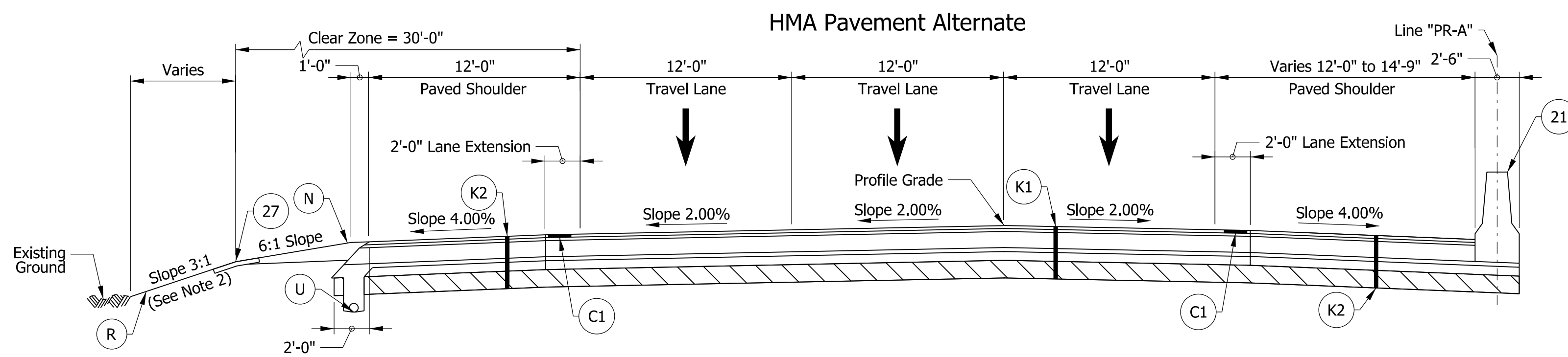
I-65 NORMAL CROWN TYPICAL SECTION STA. 824+71.00 "PR-A" to STA. 828+21.00 "PR-A"
