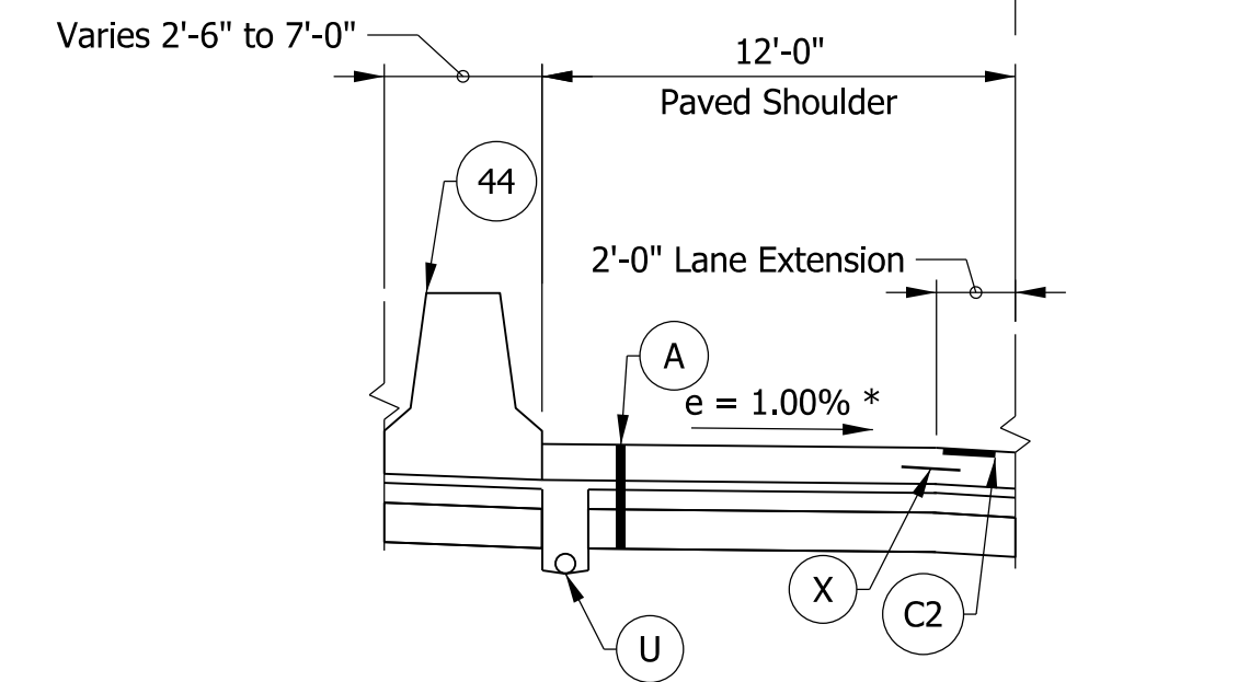
MODIFIED MEDIAN BARRIER DETAIL STA. 301+96.00 "PR-65-NB" to STA. 305+20.20 "PR-65-NB" STA. 326+08.07 "PR-65-NB" to STA. 329+61.00 "PR-65-NB"
