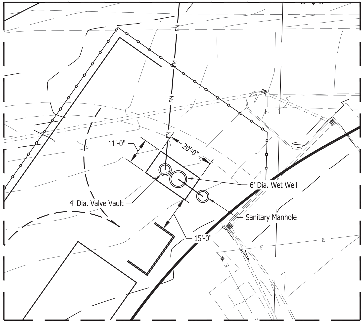
A LIFT STATION DETAILS SCALE: 1" = 20'
