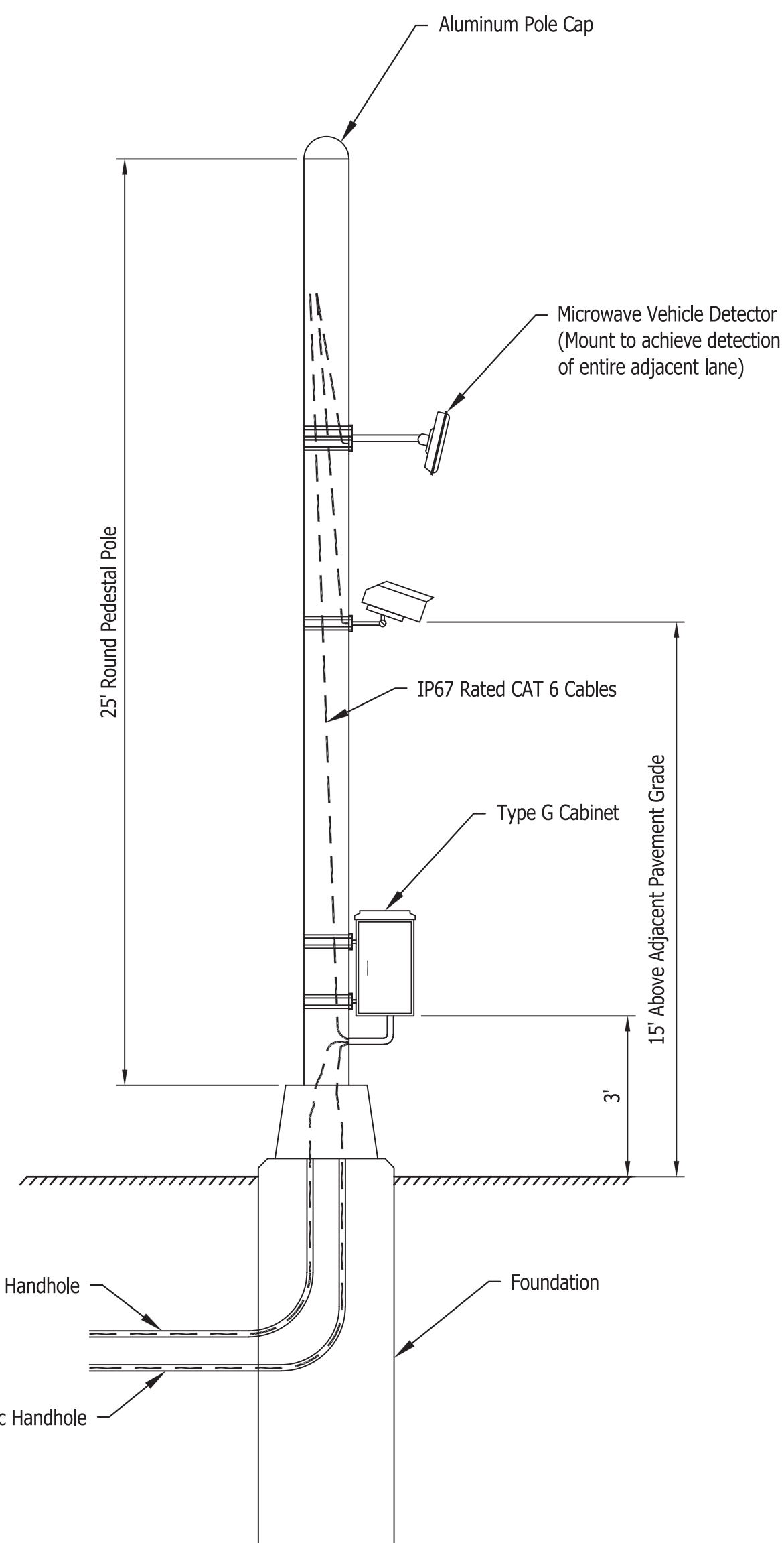
ITS VEHICLE DETECTION POLE DETAILS Not to Scale
