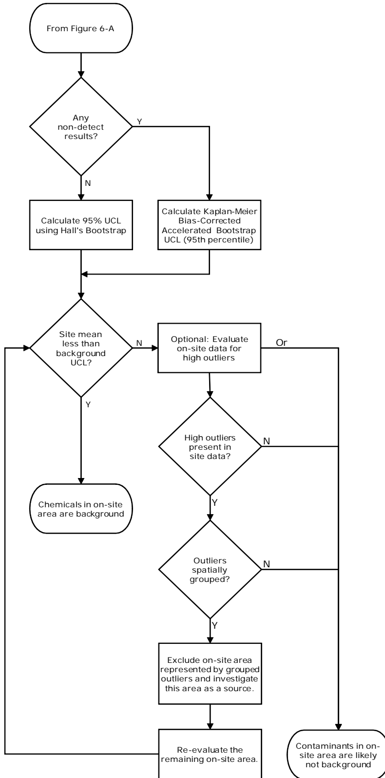
Figure 6-C: Background Evaluation under Systematic Sampling
