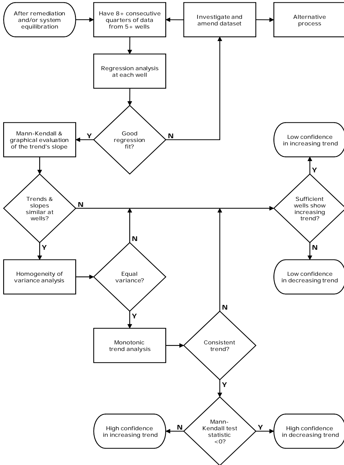
Figure 4-E: An Example of Plume Trend Analysis
