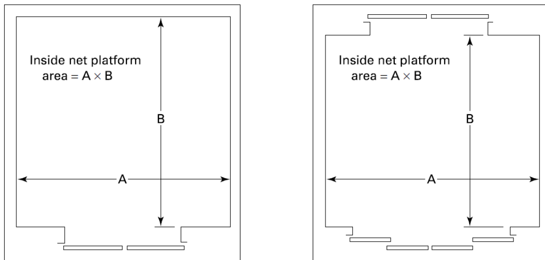
Figure 3.7.1 Inside Net Platform Areas for Passenger Elevators
