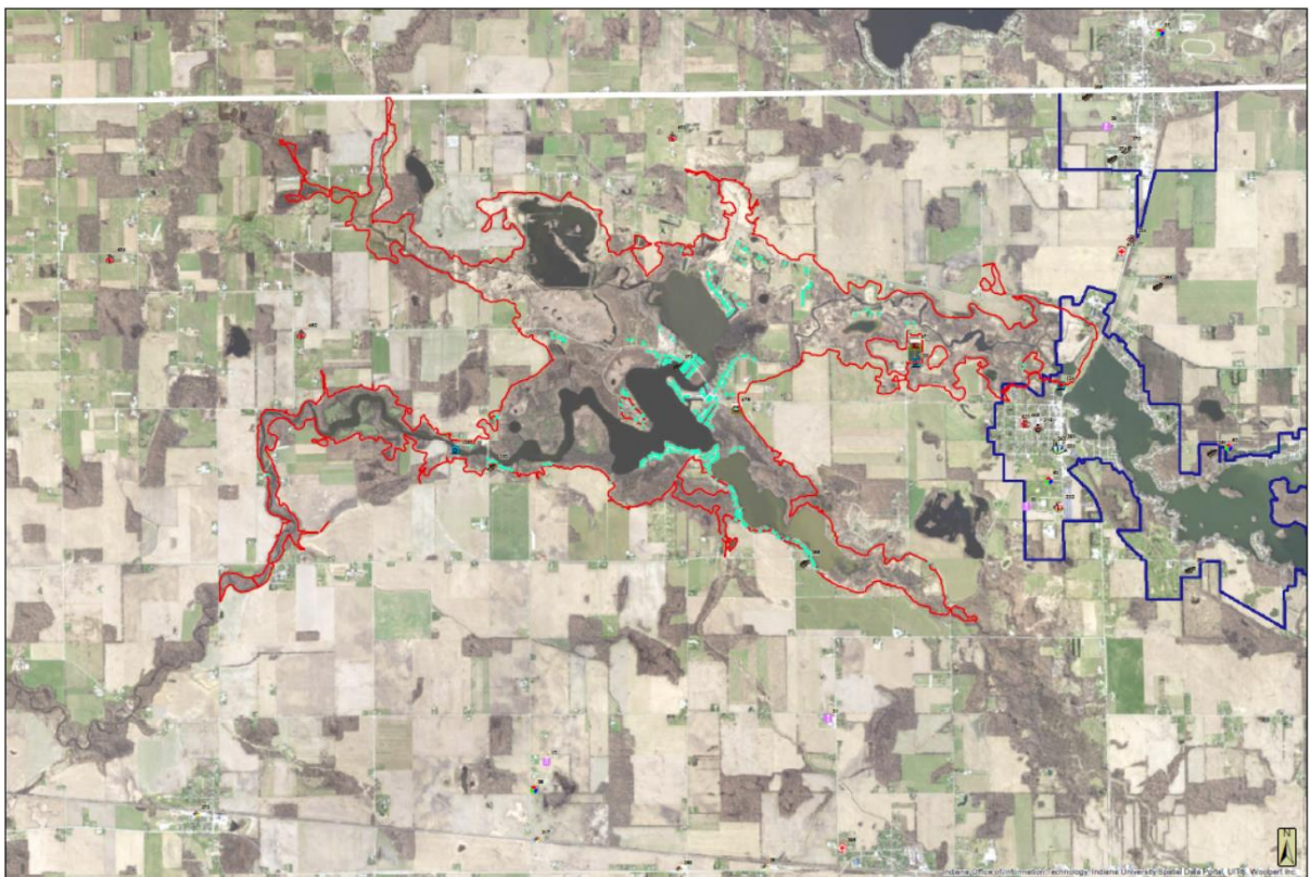
Figure 3-27 Potential Dam Failure Inundation Area, Sylvan Lake Dam
